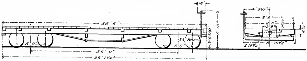
Fig. 63. Side Elevation.
